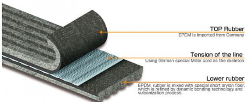
Double - sided Auxiliary drive belt,cross - section structure diagram
