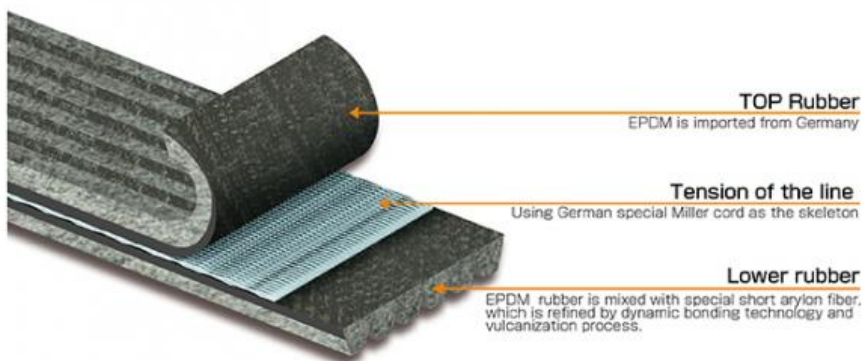
Double - sided Auxiliary drive belt,cross - section structure diagram
