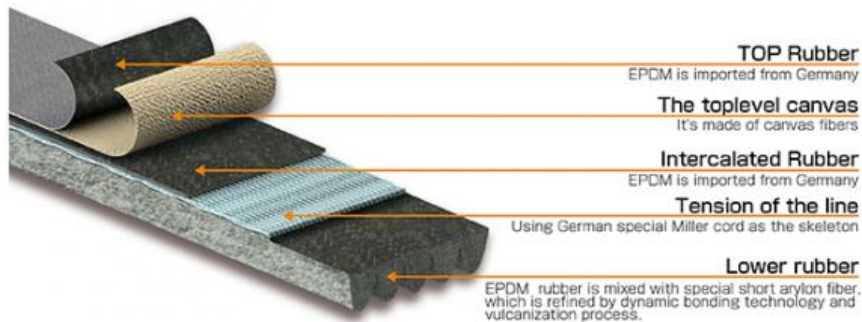
Single - sided Auxiliary drive belt,cross - section structure diagram
