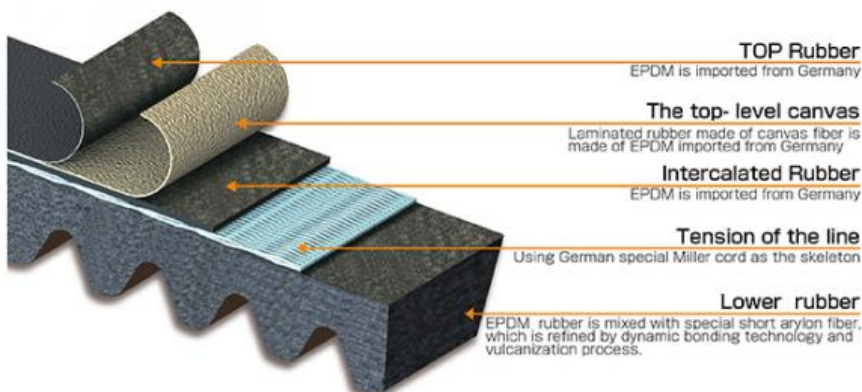
Triangular Auxiliary drive belt cross - section structure diagram
