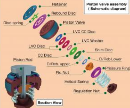
Bottom valve assembly ( Schematic diagram )
